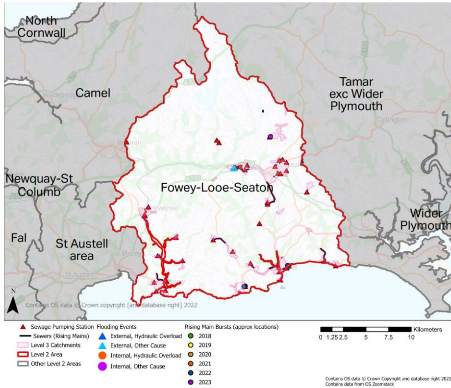
Figure 7: SPS/Rising Main flooding and burst events
