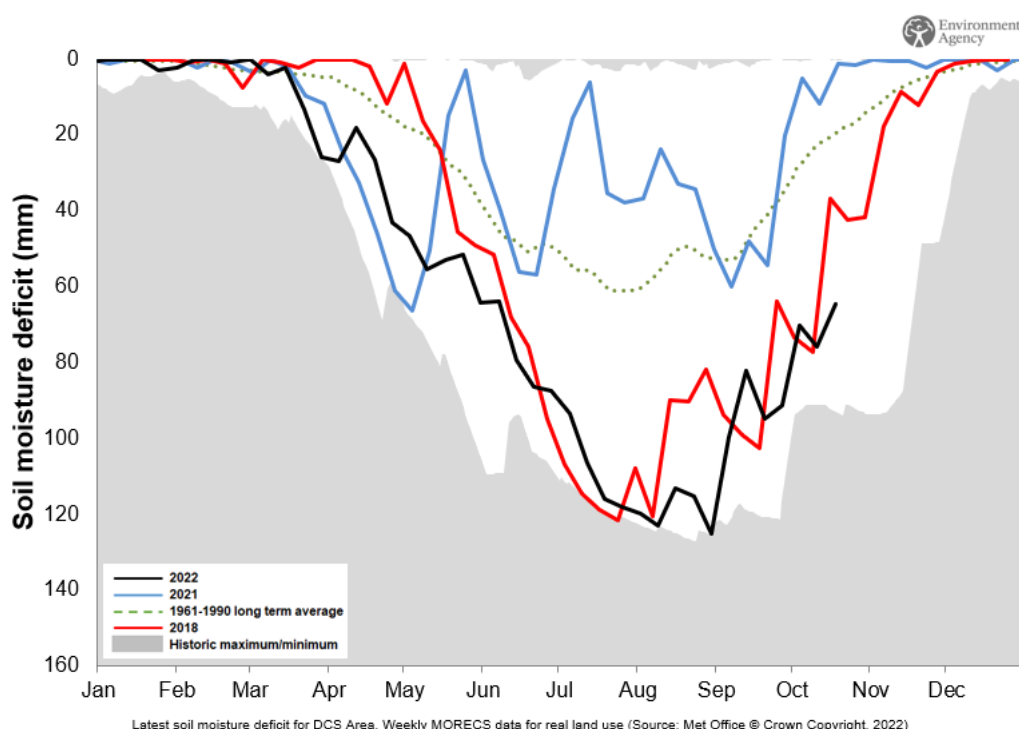
Figure 2-2: Soil Moisture Deficit for Devon and Cornwall.
