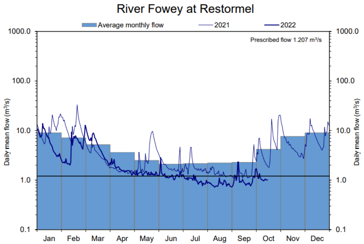
Figure 2-3: 2022 and 2021 River flow for River Fowey at Restormel from SWW's Water Situation Report.
