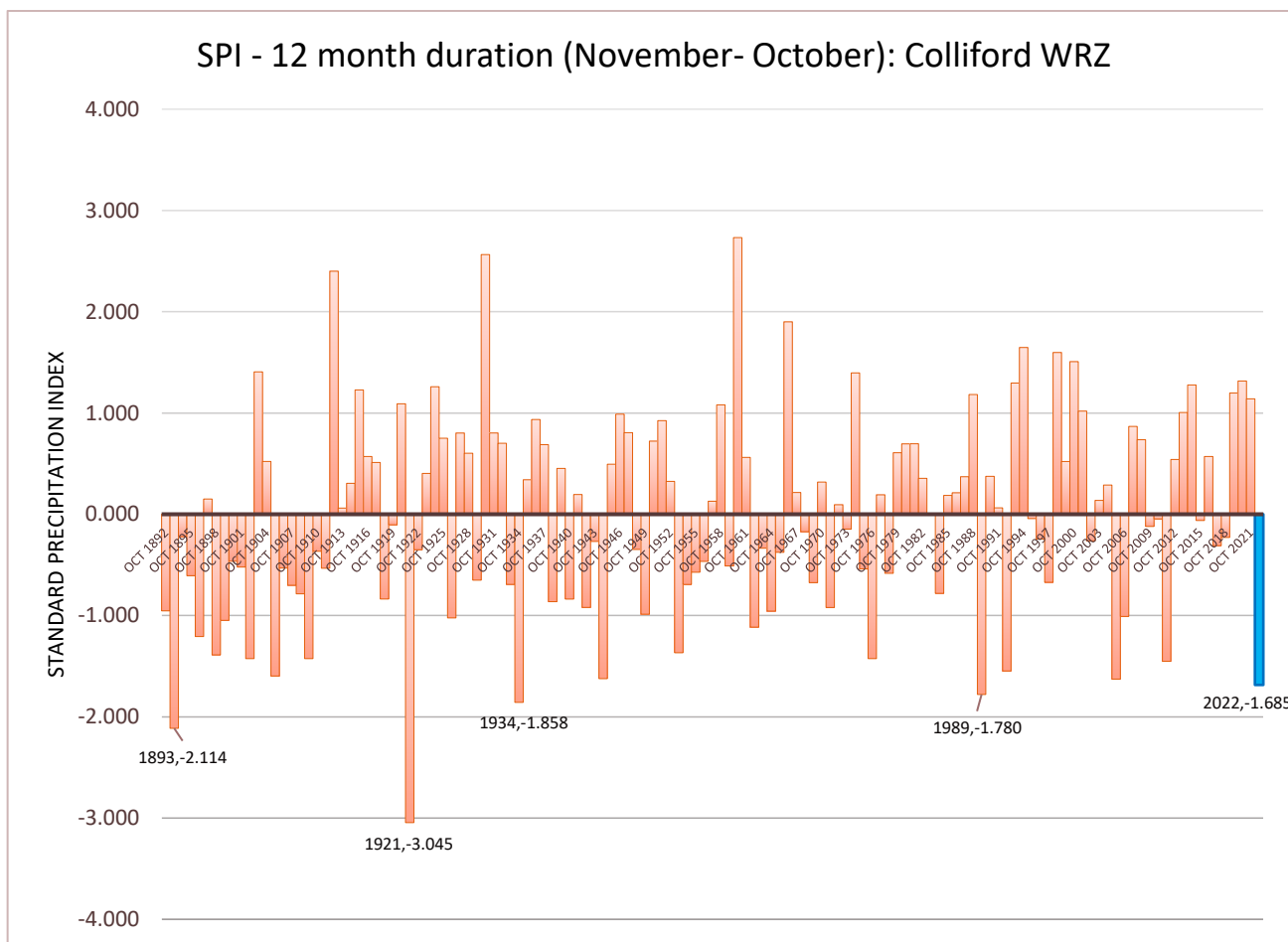
Figure 2-1: SPI values for the twelve months preceding October for the Colliford WRZ. The period of assessment is highlighted in blue
